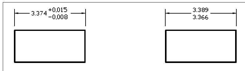
Tolerance dimension.
